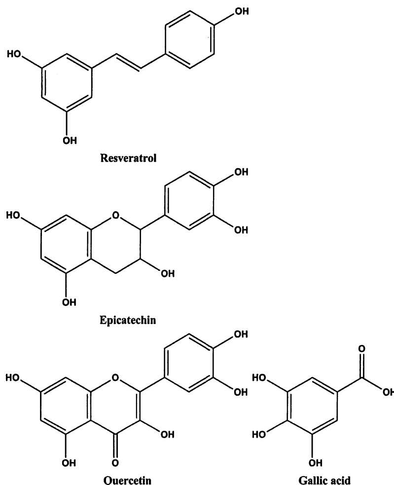
Fig. 1. Chemical structures of resveratrol, epicatechin, gallic acid, and quercetin.
