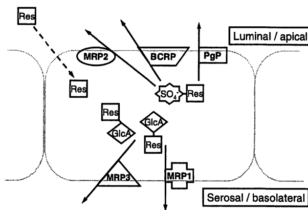
Fig. 2. Intestinal metabolism and transport of resveratrol. Resveratrol aglycone is taken up by the enterocytes, probably by passive diffusion, and is efficiently conjugated with glucuronic acid and sulfate through the action of UDP-glucuronosyl transferase and aryl-sulfatase enzymes. Methylation has not been observed, presumably due to the lack of a catechol function in the resveratrol molecule, which is a requirement for catechol-O-methyltransferase (COMT). The conjugates are transported out of the enterocytes by as yet unconfirmed processes, but it is thought that efflux transporters of the multi-drug resistance proteins (MRP) family are involved (several are indicated). Resveratrol sulfate is preferentially transported to the apical (luminal) side of polarized enterocytes, while resveratrol glucuronides are preferentially effluxed to the basolateral (serosal) side (Kaldas et al., 2003). Hence, the predominant form of resveratrol in human blood following oral dosing is resveratrol glucuronide (95 to 99% of total plasma resveratrol). Solid arrows, probable active transport process; dashed arrows, diffusion; Res, resveratrol; GlcA, glucuronic acid; SO 4 2- , sulfate; MRP, multi-drug-resistance protein; BCRP, breast cancer resistance protein; PgP, P-glycoprotein.
